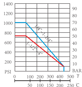
Pressure-Temperature Rating 1/4"~4"
